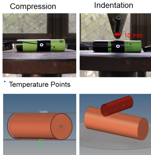
Figure 5 – Test setup &amp; structural simulation models
