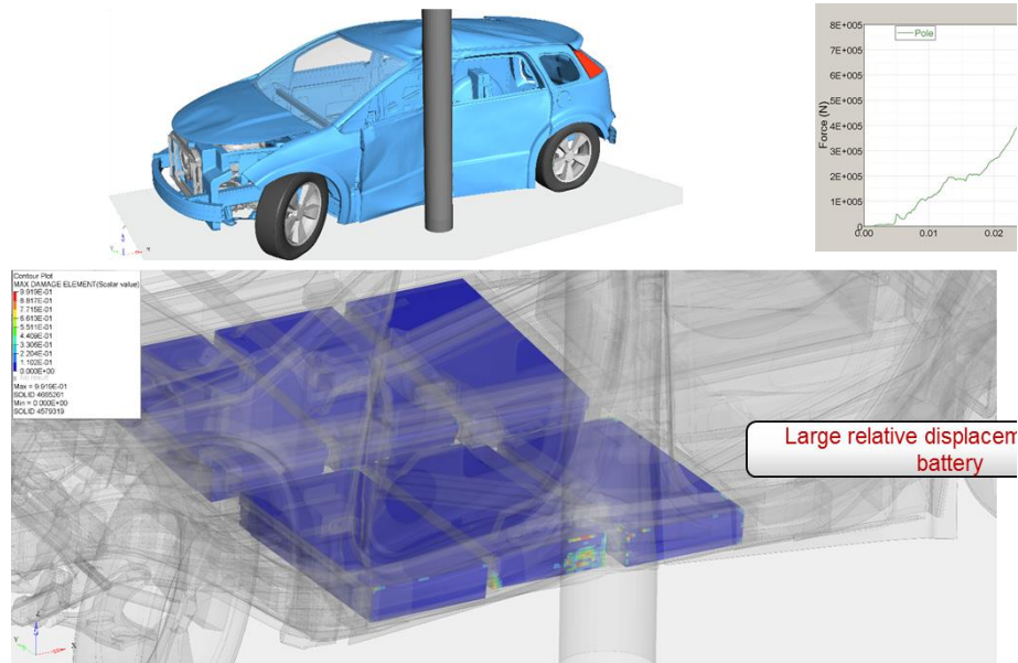
Figure 2 – Battery mechanical response to a vehicle pole impact
