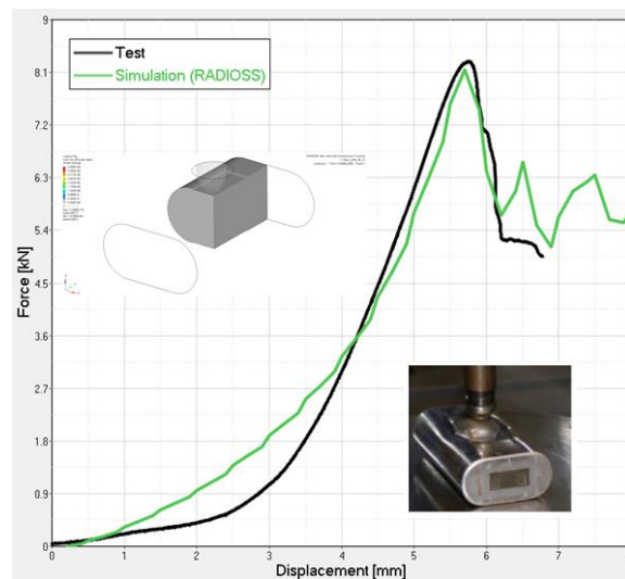
Figure 1 – Simulation vs test results of a battery cell hemispherical indentation
