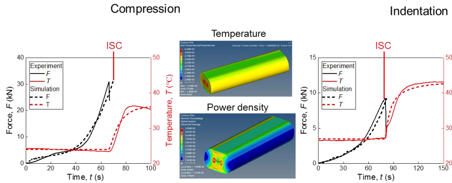
Figure 7 – Numerical results vs experimental curve
